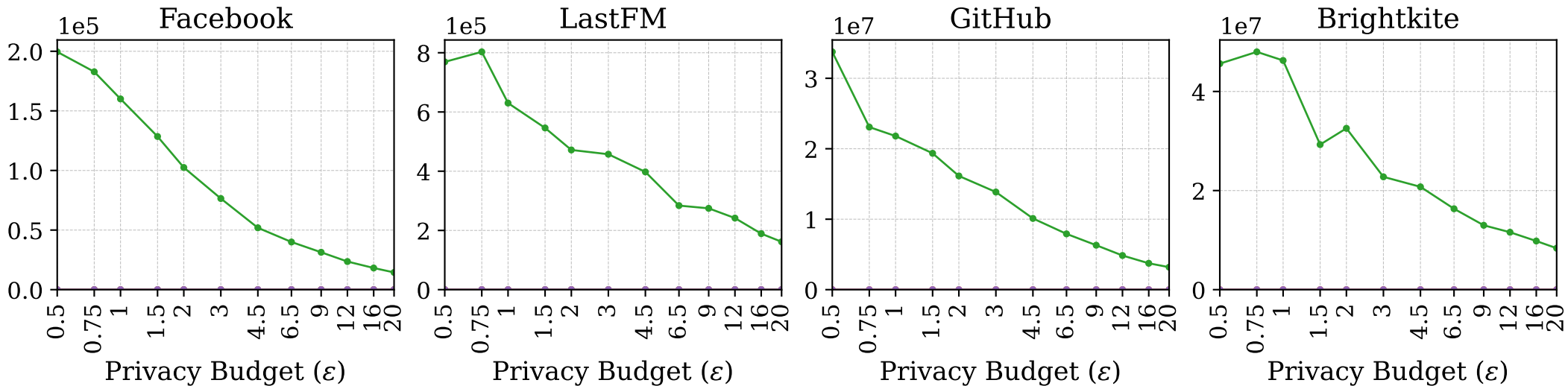
(h) Harmonic Diameter Error
